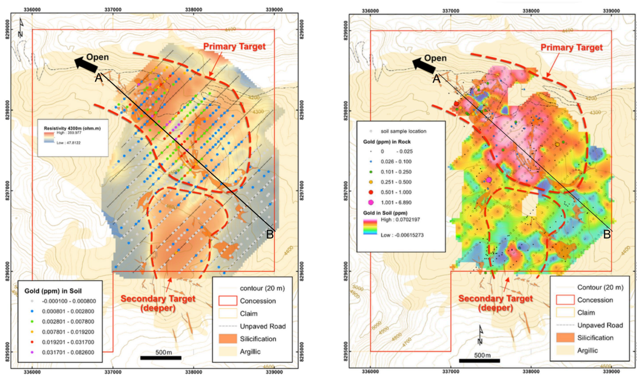
Figure 7. Pucarini Project: Soil geochemistry coincident with a high resistivity anomaly
