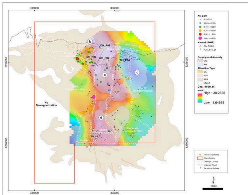
Figure 6. Map of Pucarini Project, Peru showing a summary of key exploration targeting evidence and proposed drill hole locations. A high chargeability anomaly coincides with a high resistivity and soil and rock geochemistry.
