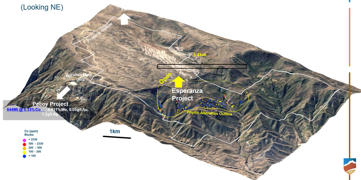
Figure 3. Esperanza Project property geology map showing prominent crustal structural break that controls Pecoy-Esperanza-Andaray Cu-Mo porphyry corridor.
