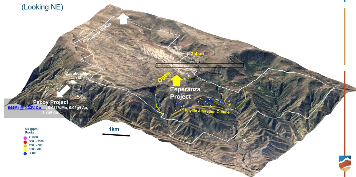
Figure 3. Esperanza Project property geology map showing a prominent crustal structural break that controls Pecoy-Esperanza-Andaray Cu-Mo porphyry corridor.
